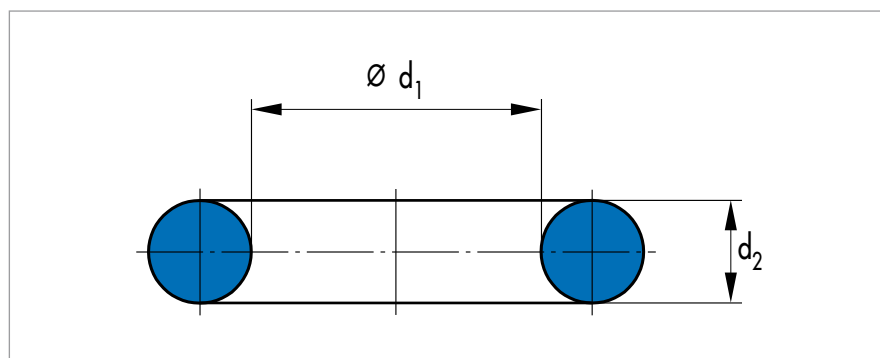
Fig. 2 Drawing with dimensions
